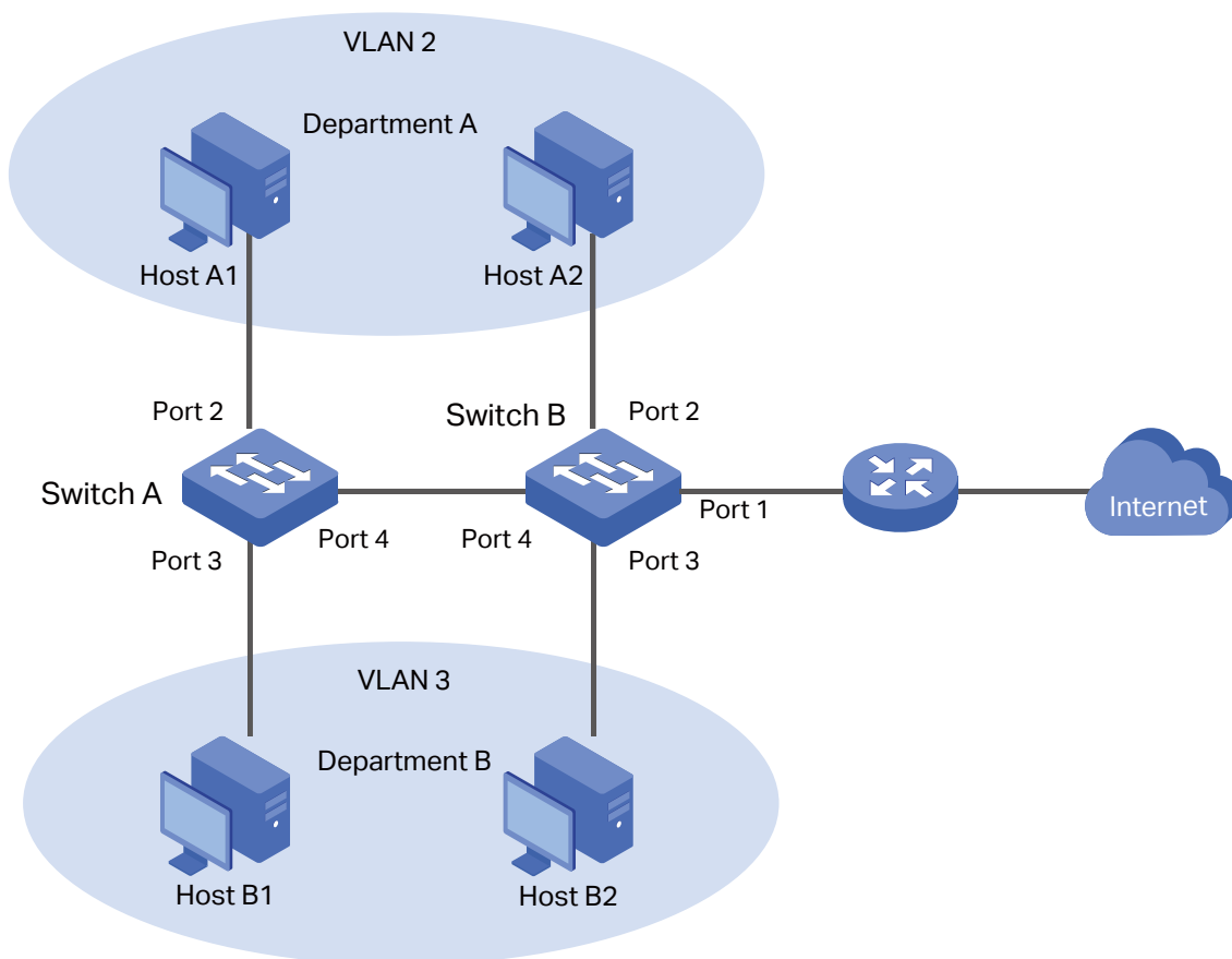
Figure 5-1 Network Topology
