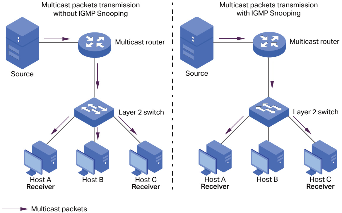
Figure 1-1 IGMP Snooping
